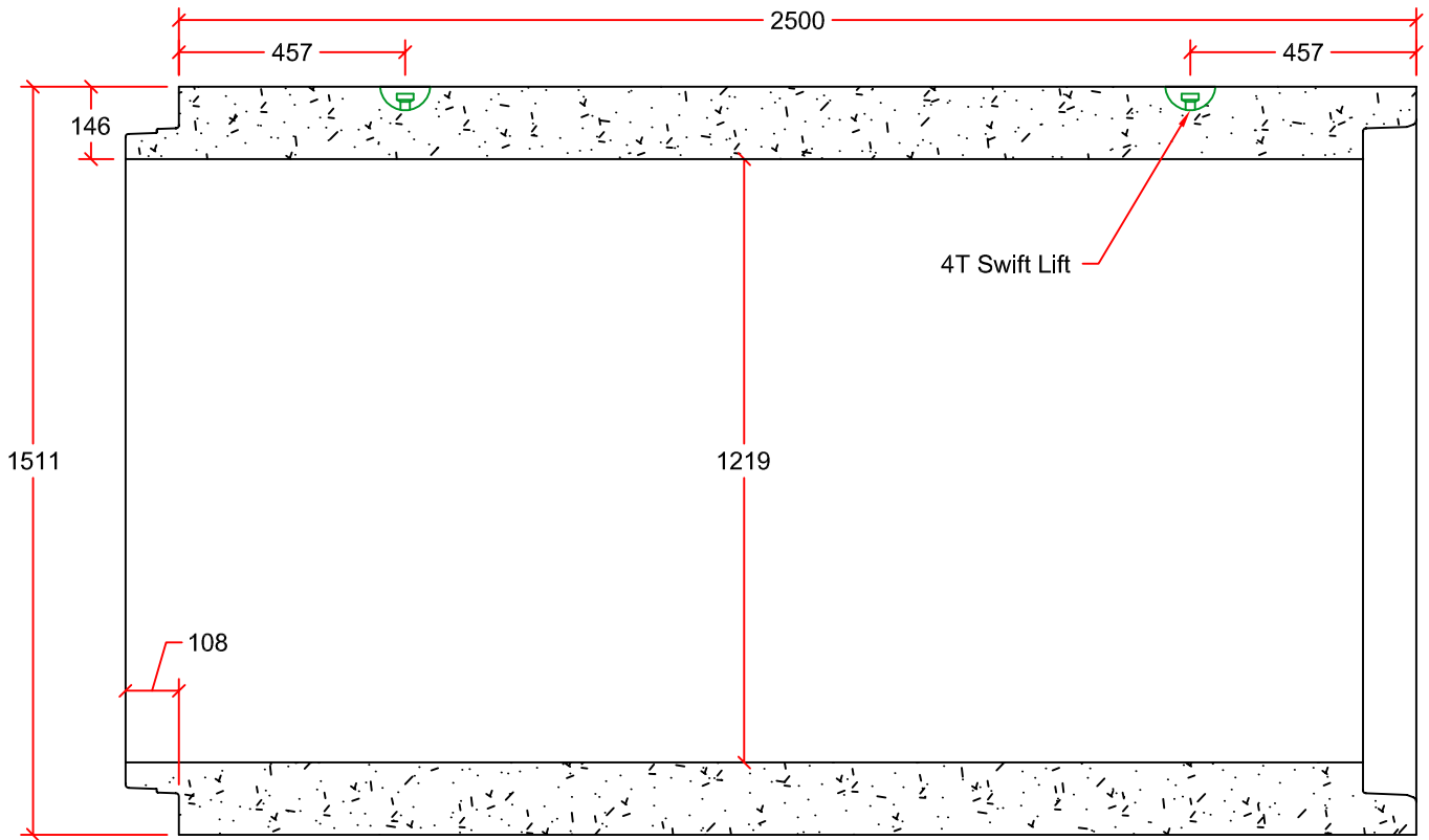
PIPE DETAIL
