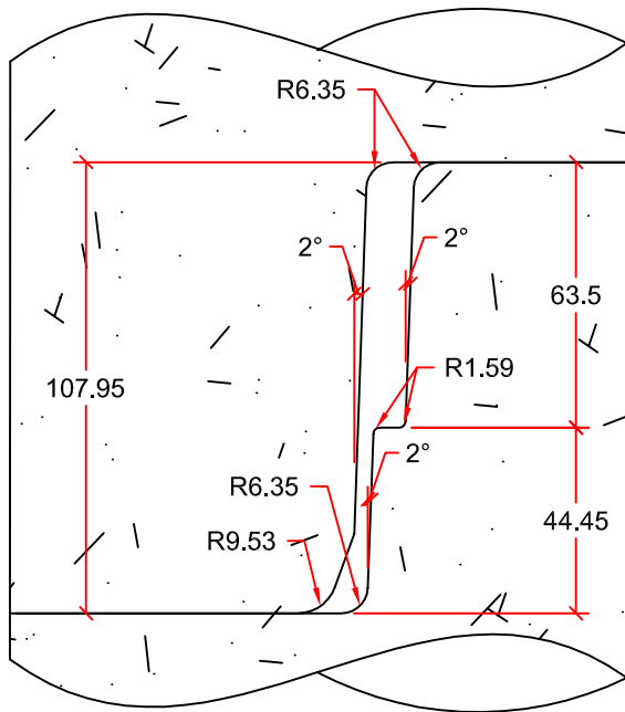
JOINT DETAIL
