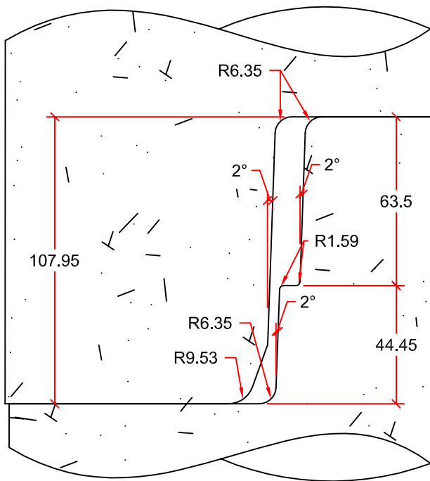
JOINT DETAIL
