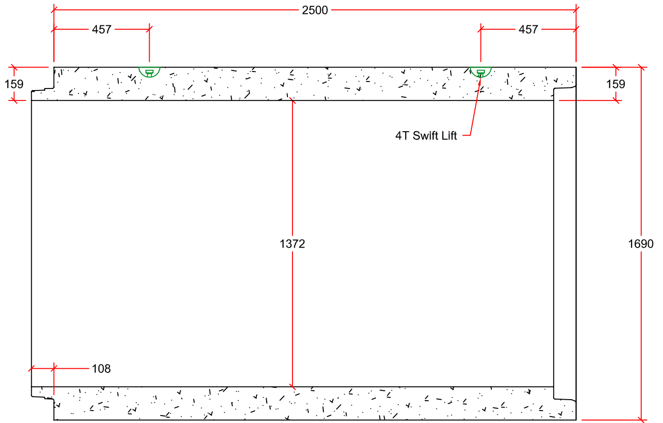
PIPE DETAIL
