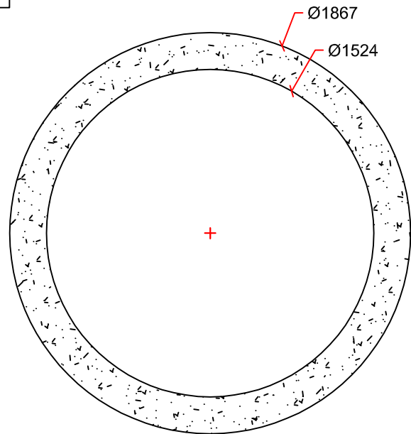
SECTION DETAIL
