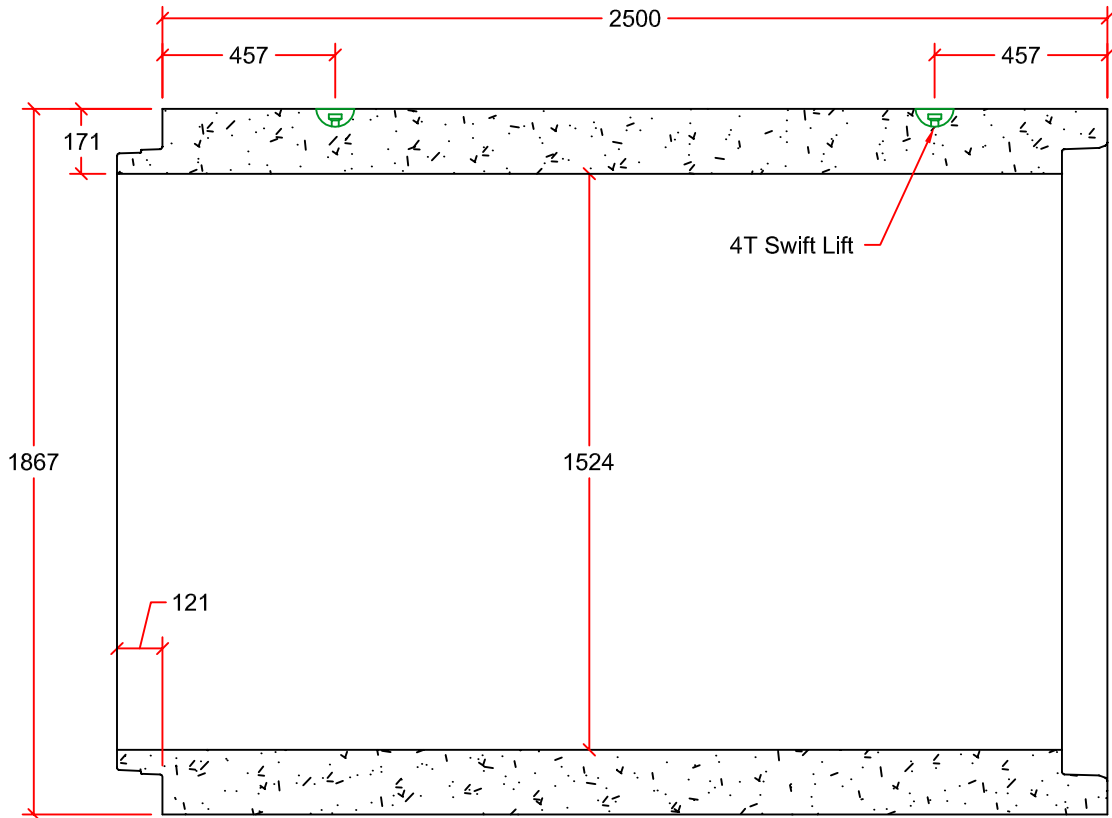
PIPE DETAIL
