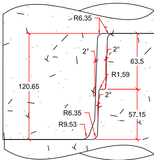
JOINT DETAIL
