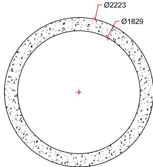
SECTION DETAIL
