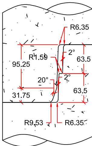
JOINT DETAIL
