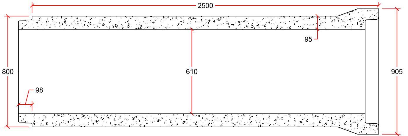
PIPE DETAIL
