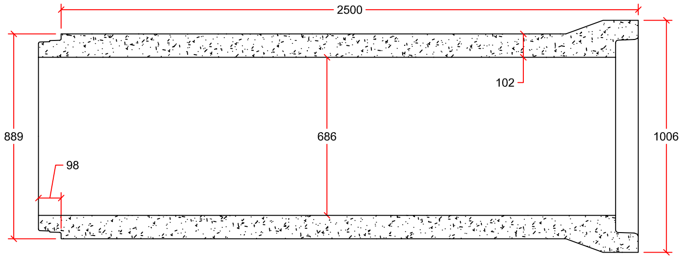
PIPE DETAIL
