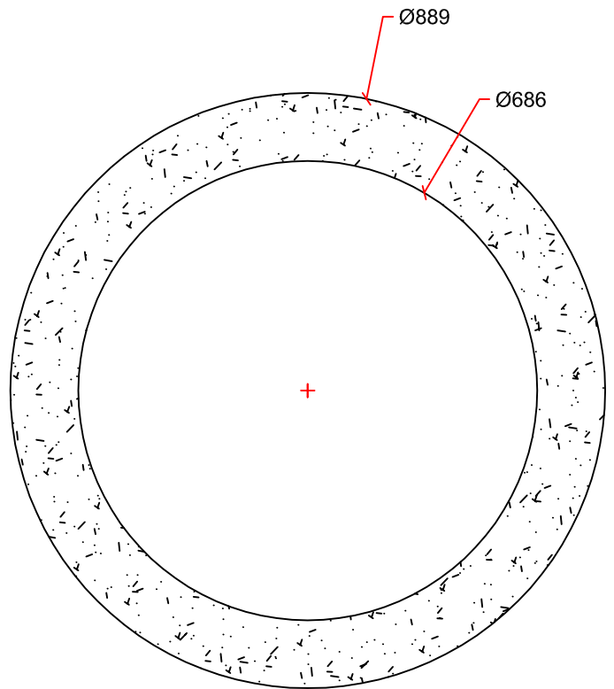
PIPE DETAIL
