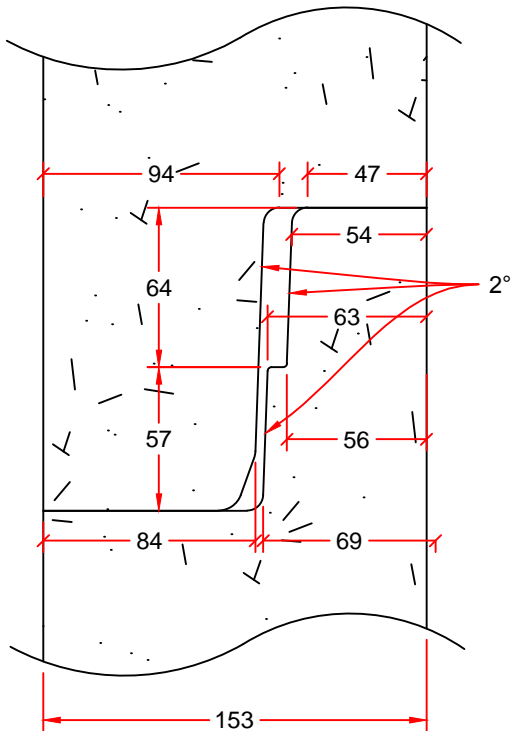
JOINT DETAIL
