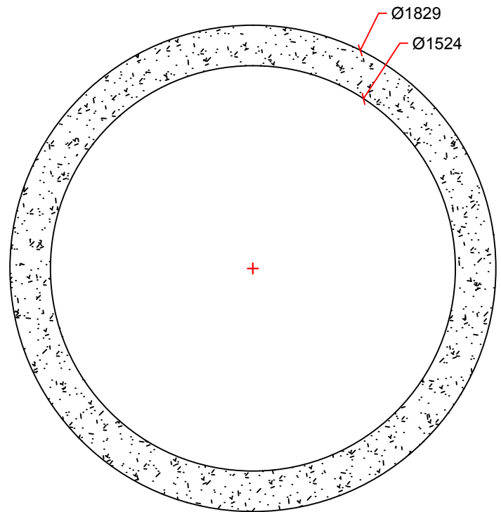
SECTION DETAIL
