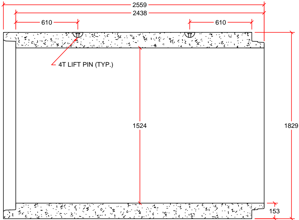
PIPE DETAIL
