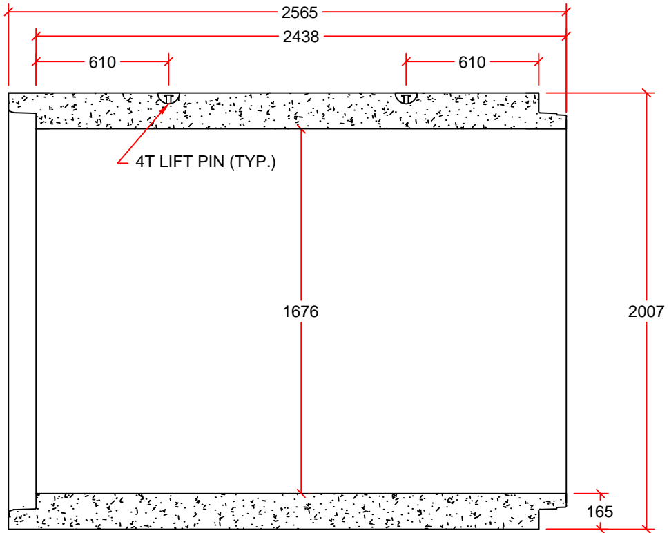
PIPE DETAIL
