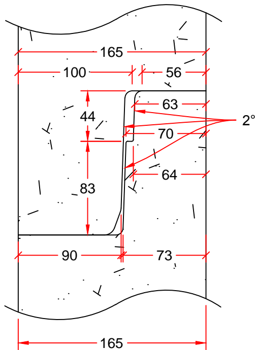
JOINT DETAIL
