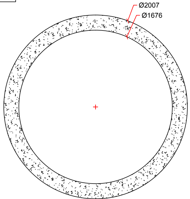
PIPE DETAIL
