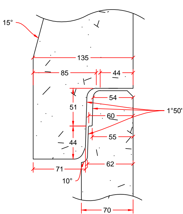
JOINT DETAIL
