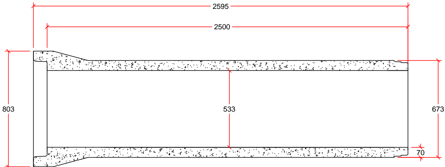
PIPE DETAIL
