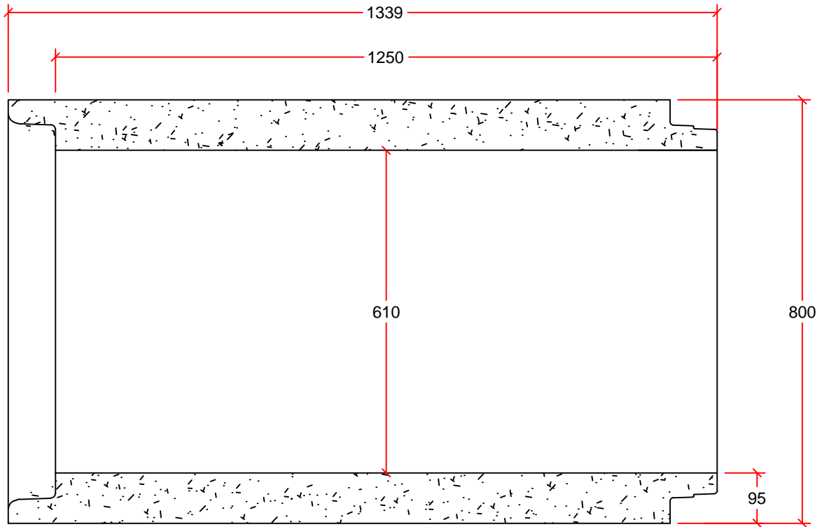
PIPE DETAIL
