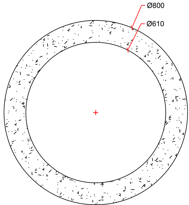
SECTION DETAIL
