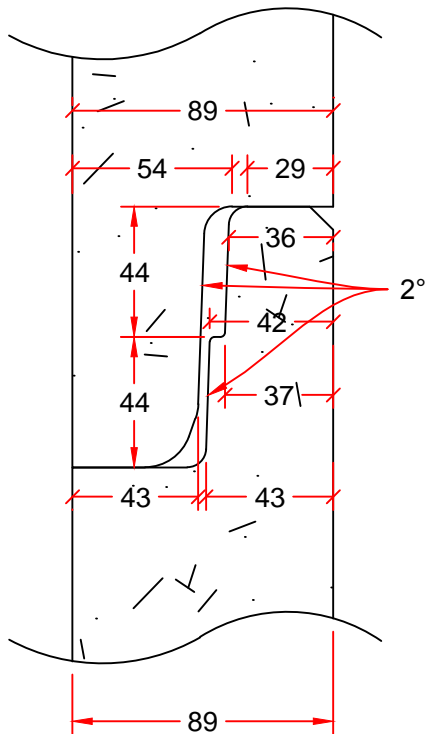
JOINT DETAIL
