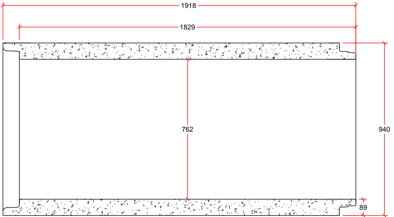
PIPE DETAIL
