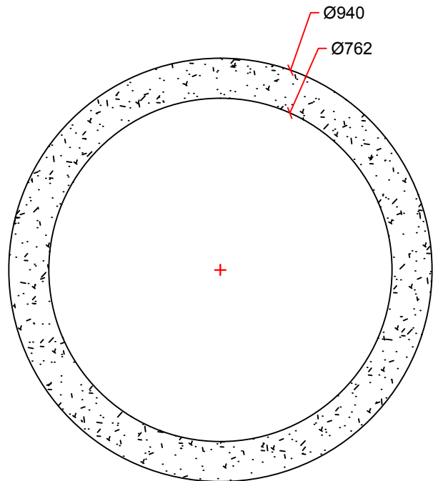
SECTION DETAIL
