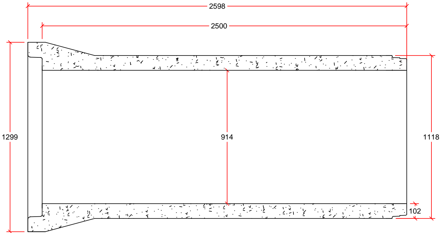
PIPE DETAIL
