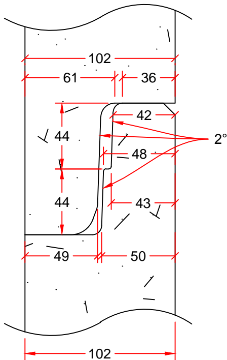
JOINT DETAIL
