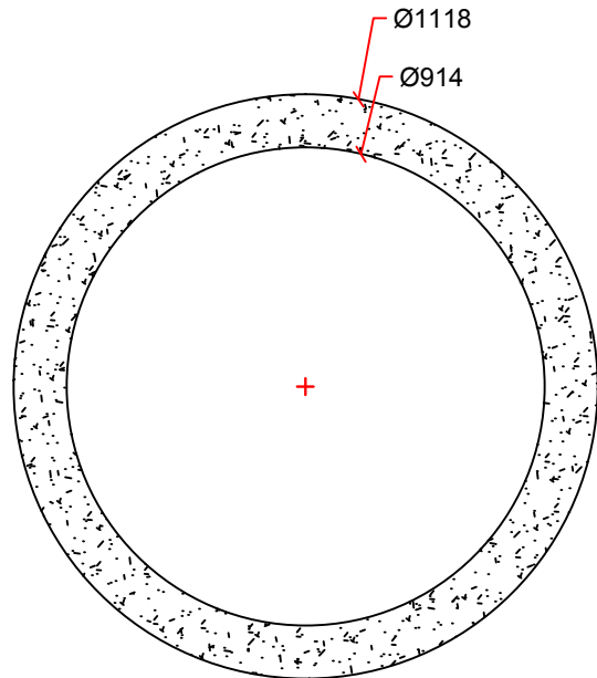
SECTION DETAIL
