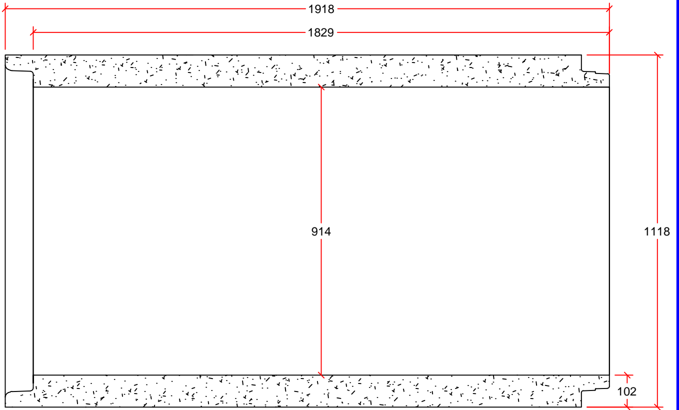
PIPE DETAIL
