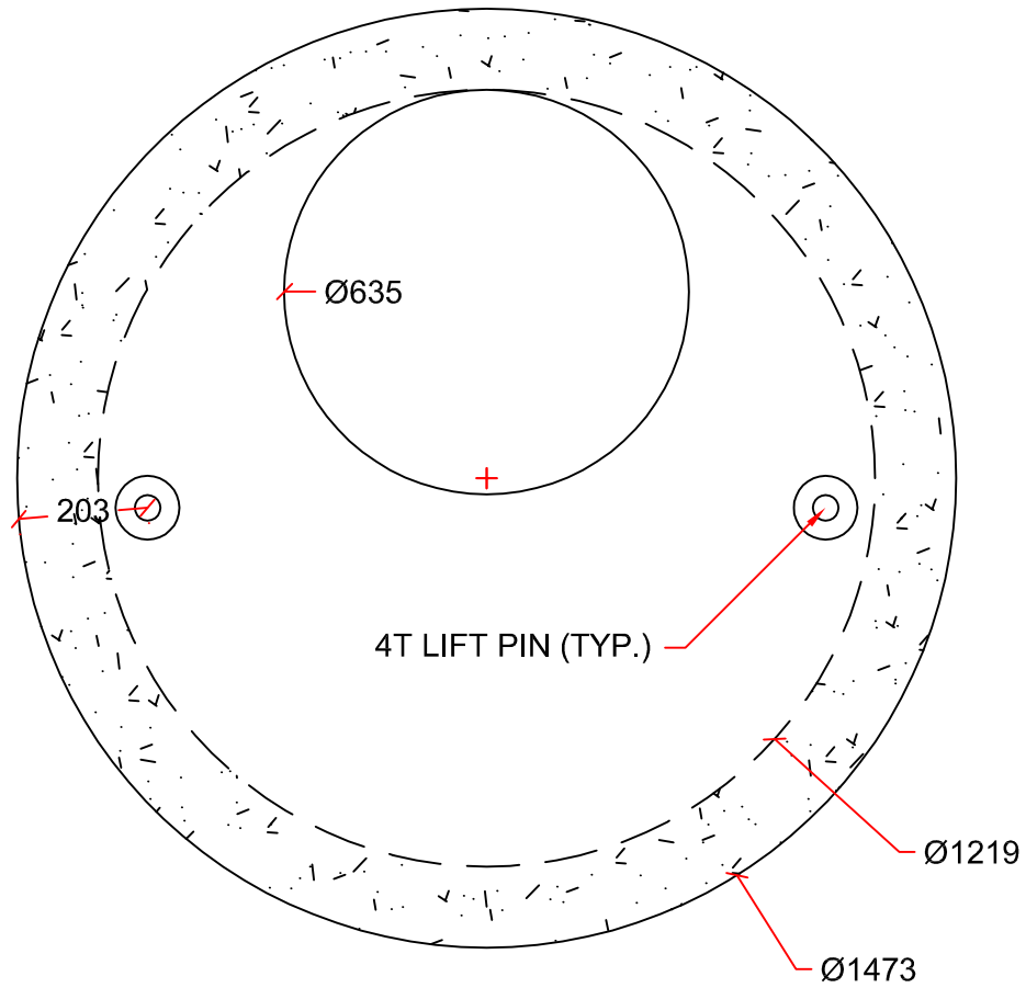
PLAN VIEW
