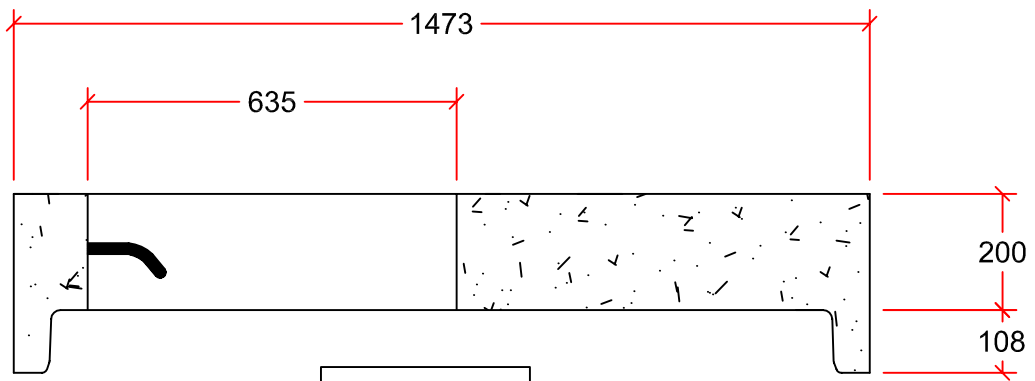
PROFILE VIEW
