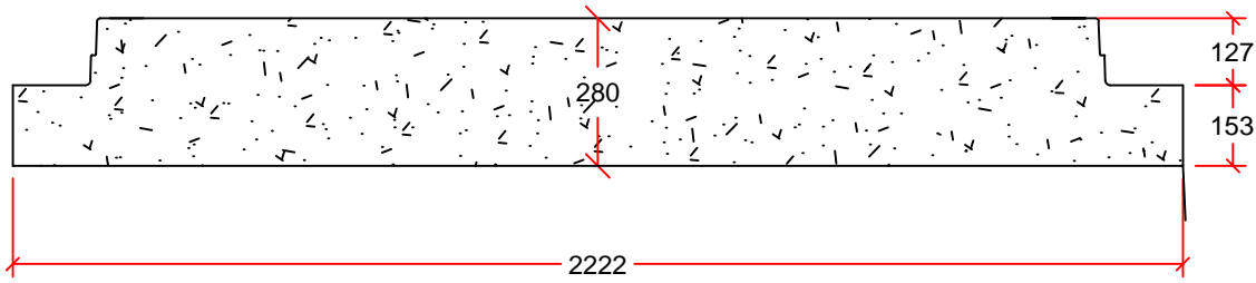
PROFILE VIEW
