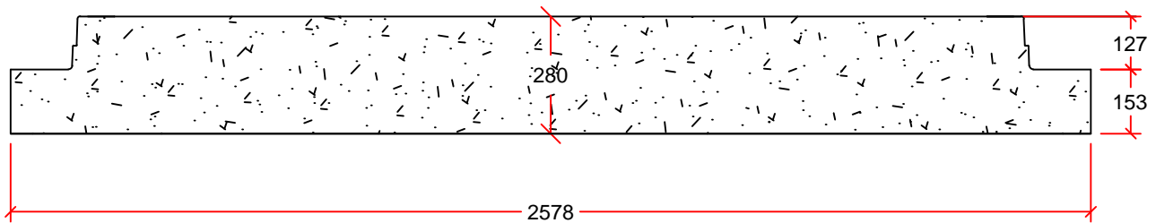
PROFILE VIEW
