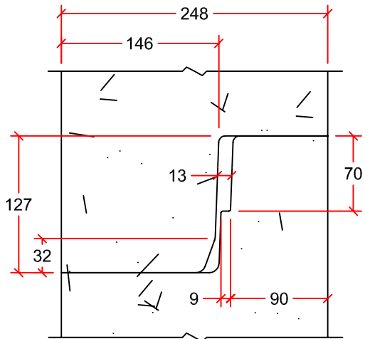
JOINT DETAIL
