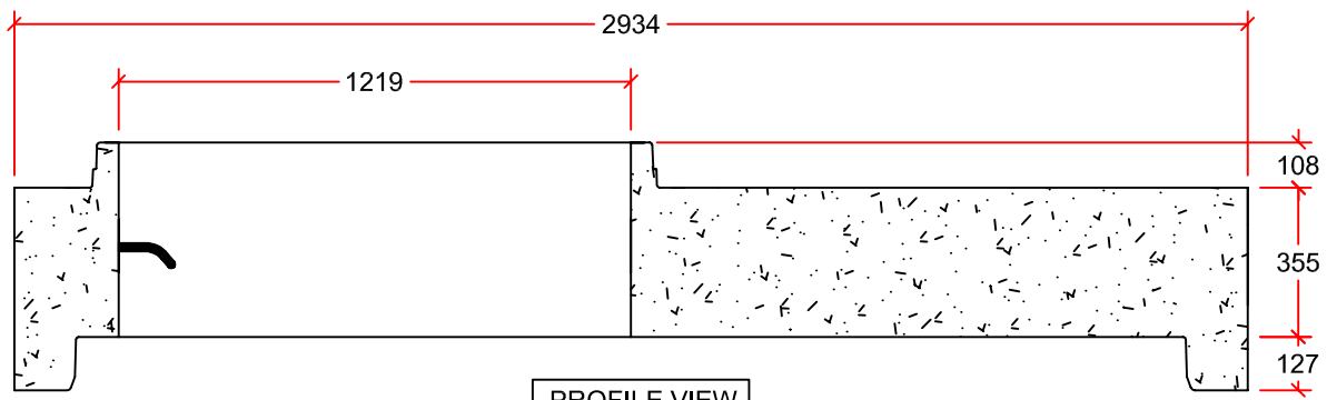
PROFILE VIEW
