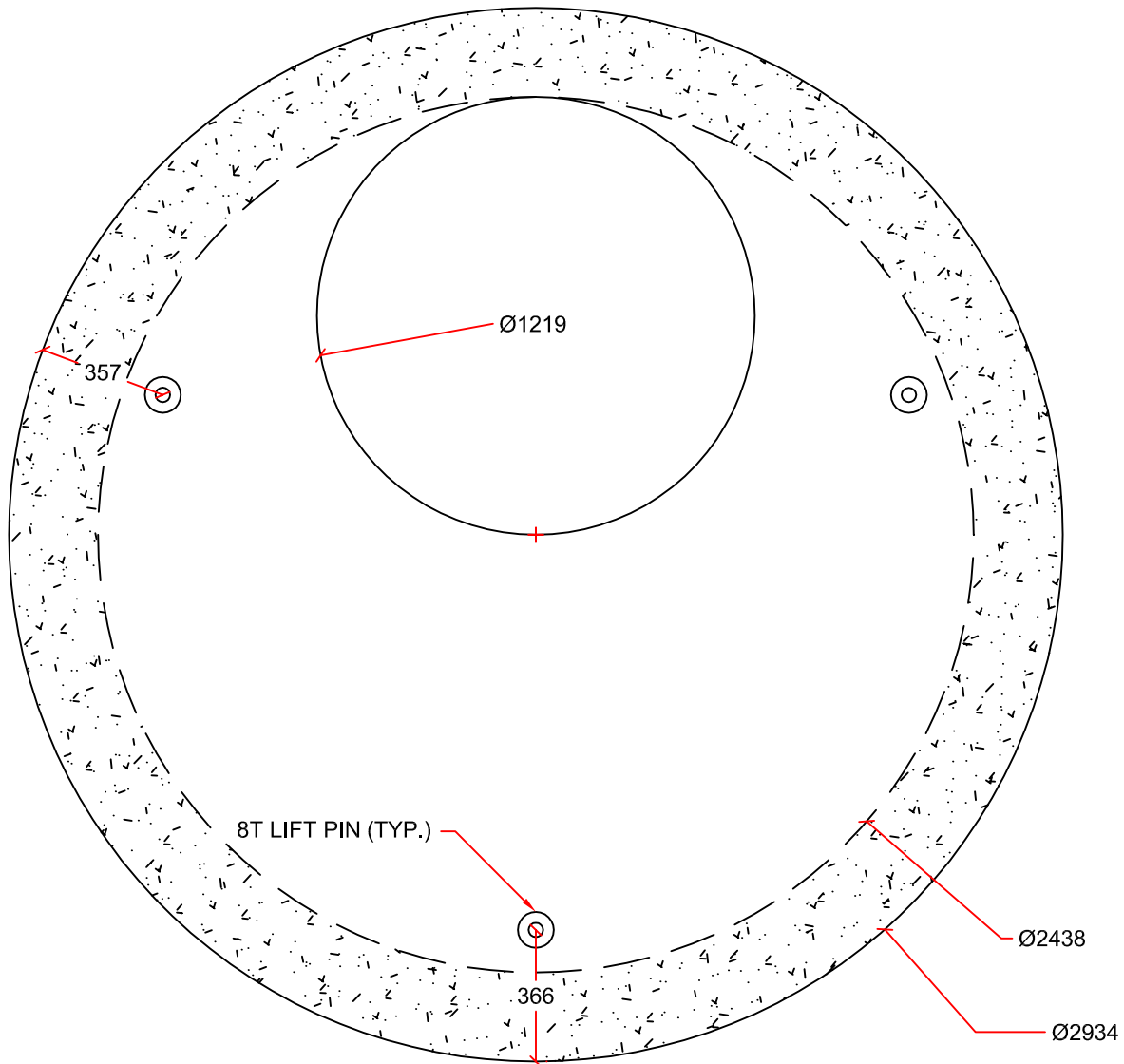
PLAN VIEW
