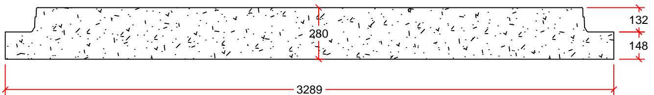
PROFILE VIEW
