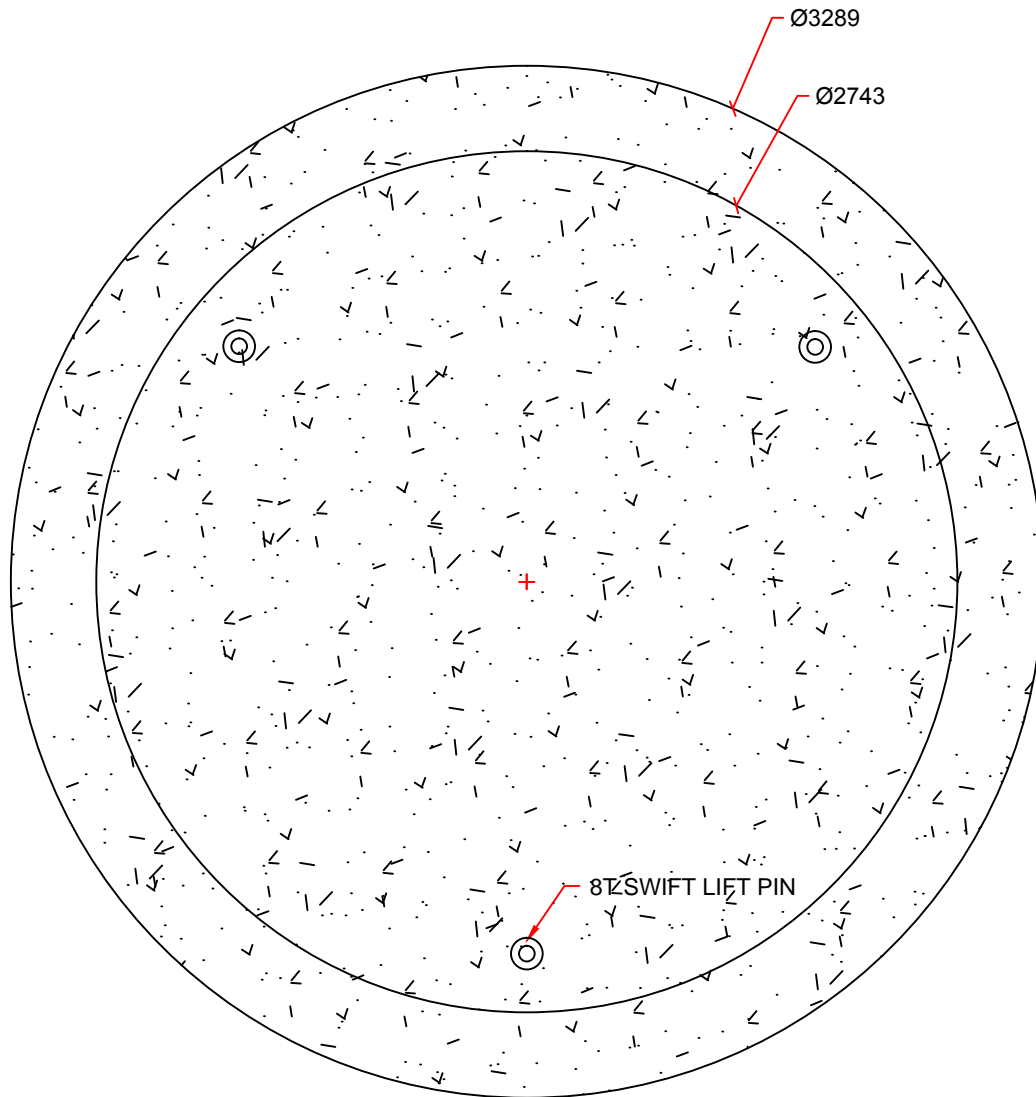
PLAN VIEW
