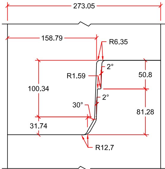
JOINT DETAIL
