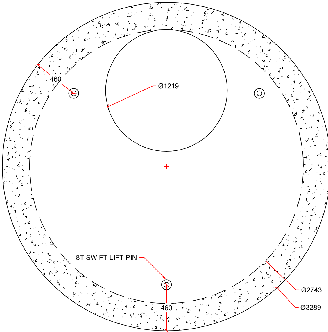
PLAN VIEW
