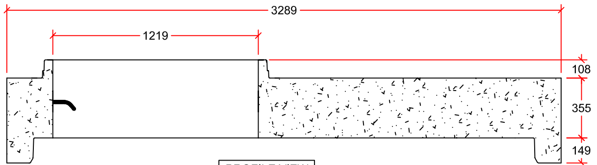
PROFILE VIEW
