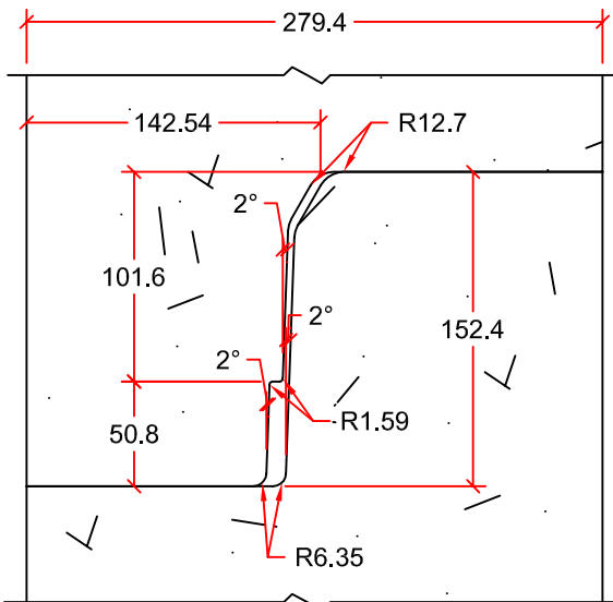
JOINT DETAIL
