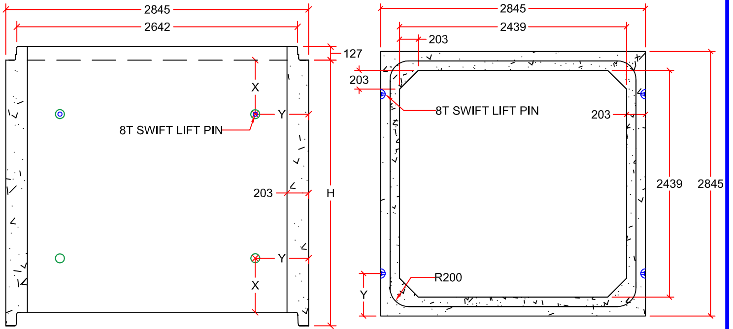
PROFILE VIEW
