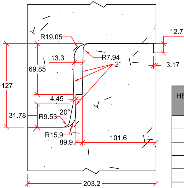
JOINT DETAIL
