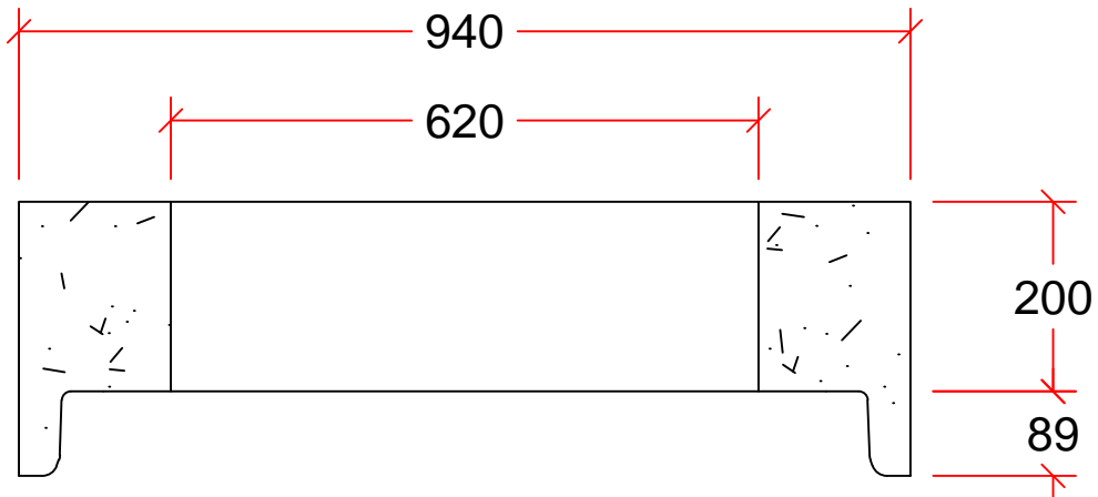
750mm SLAB TOP W/ 620mm SQUARE OPENING
