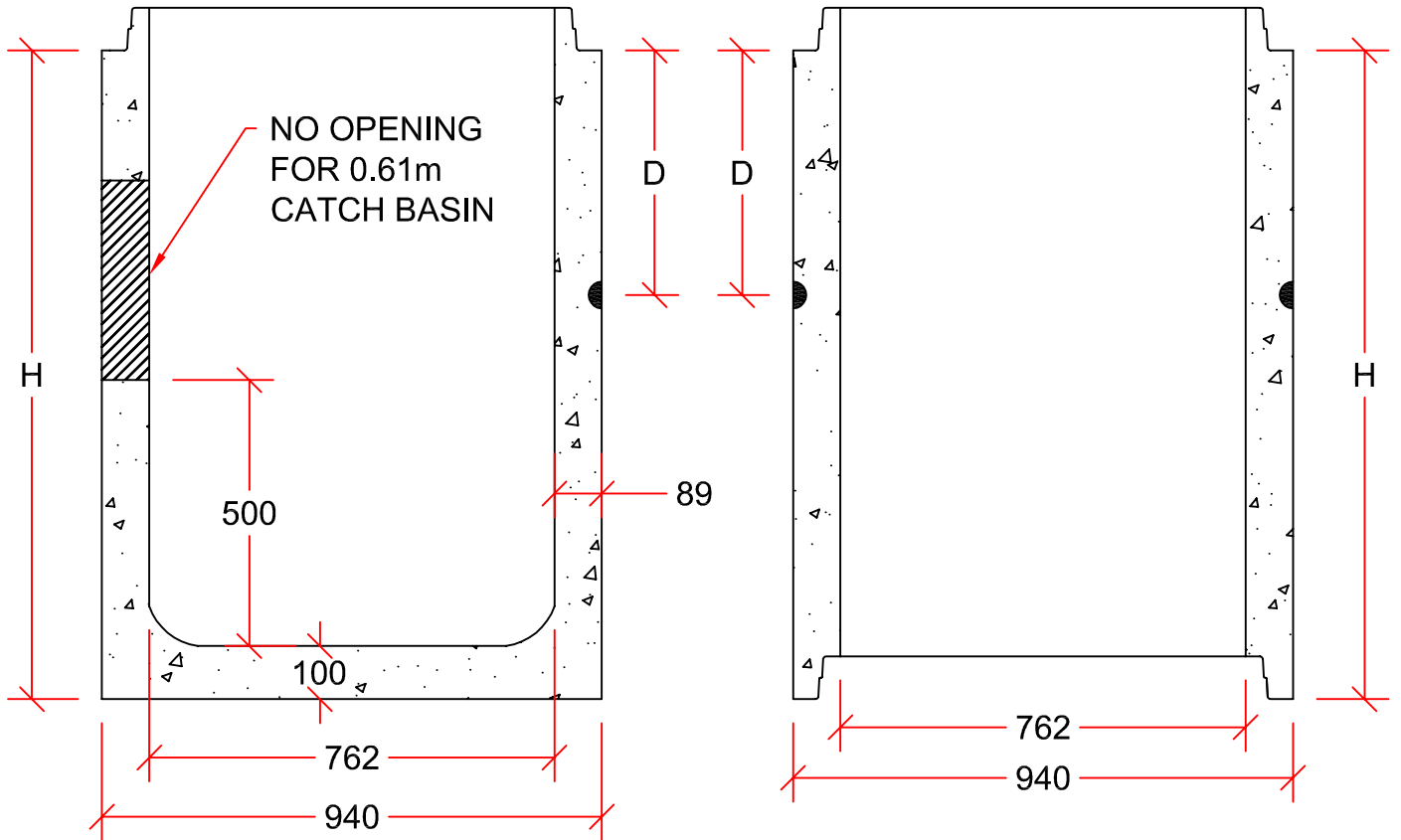
CATCH BASINS AVAILABLE IN 0.61m, 1.22m, AND 1.83m HEIGHTS
