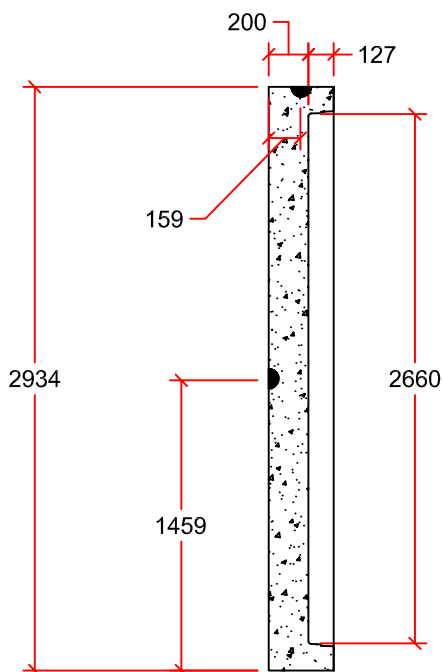
PROFILE VIEW
