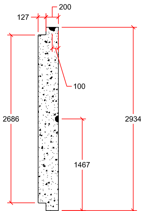
PROFILE VIEW
