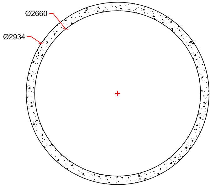
SECTION DETAIL
