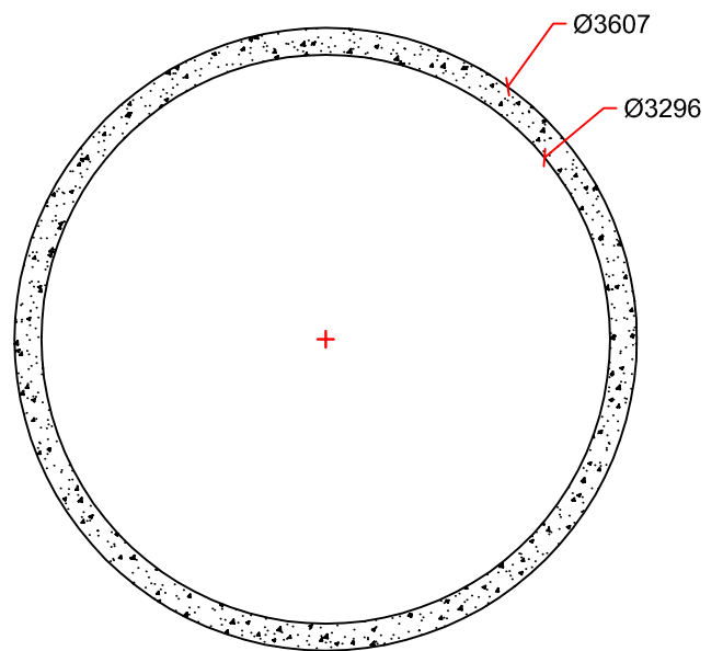
SECTION DETAIL
