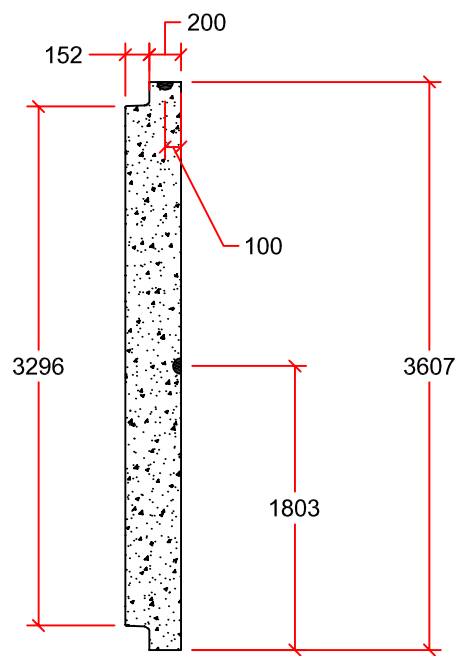
PROFILE VIEW
