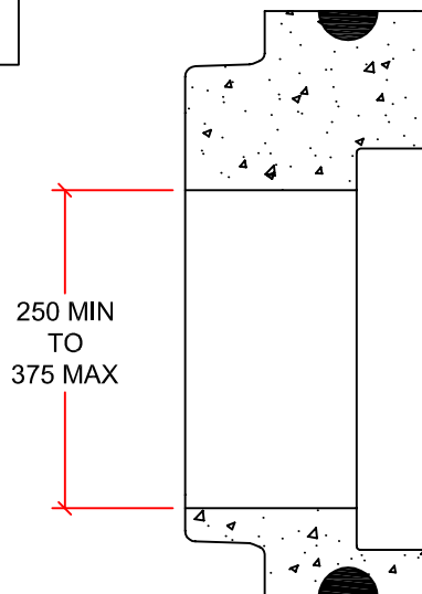
INCREASER
