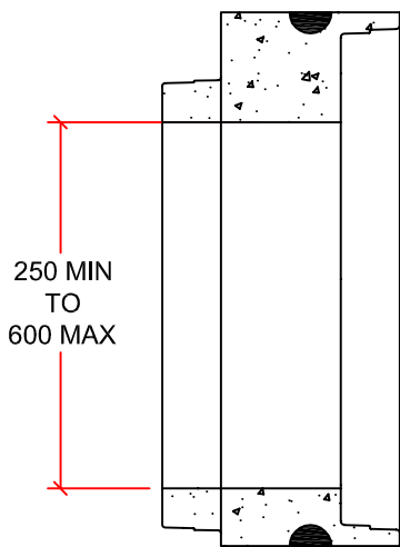
SECTION DETAIL
