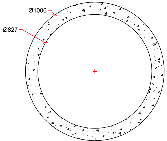
SECTION DETAIL
