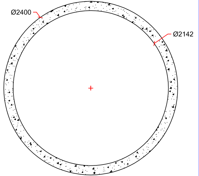
SECTION DETAIL
