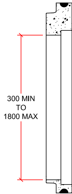
INCREASER
