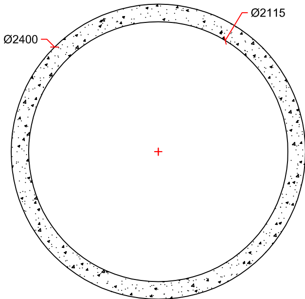
SECTION DETAIL
