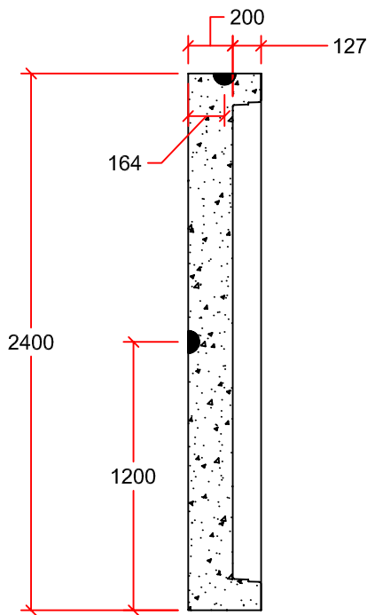
PROFILE VIEW
