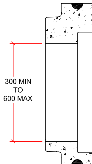
INCREASER
