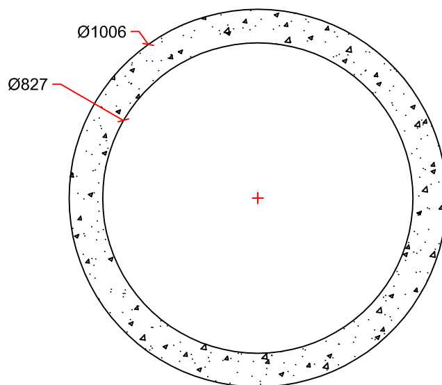
SECTION DETAIL
