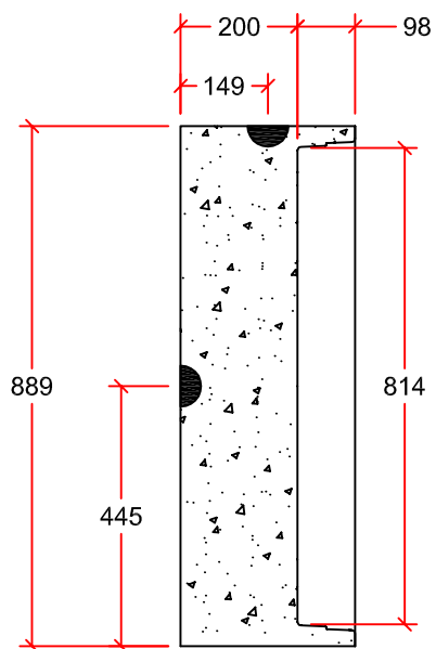
PROFILE VIEW
