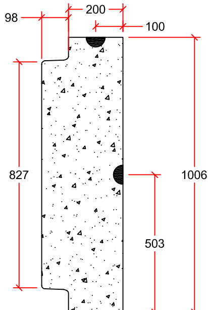
PROFILE VIEW
