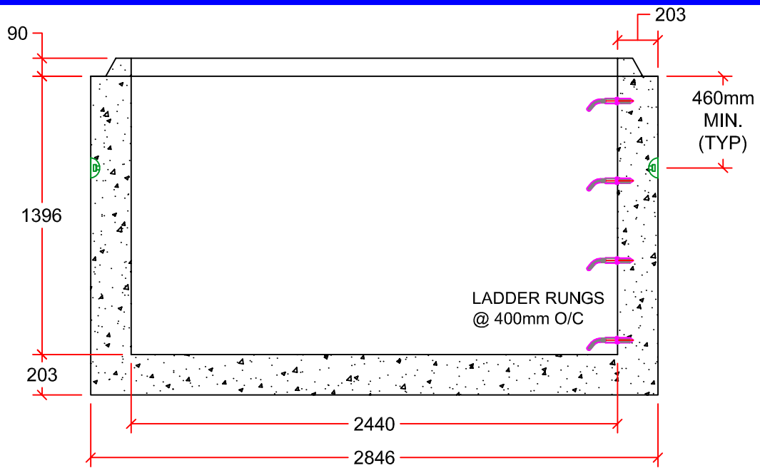
SIDE VIEW
