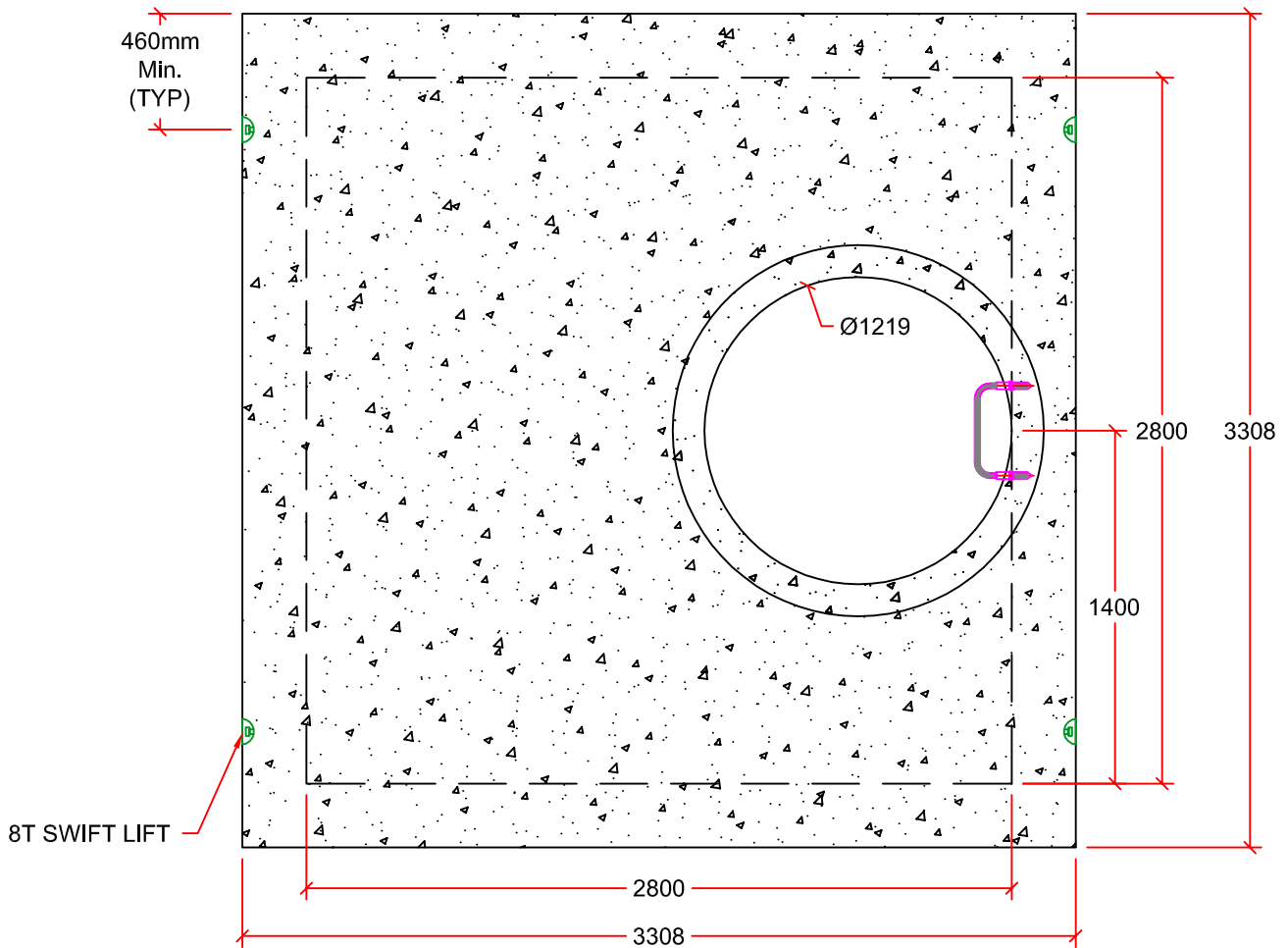
TOP VIEW
